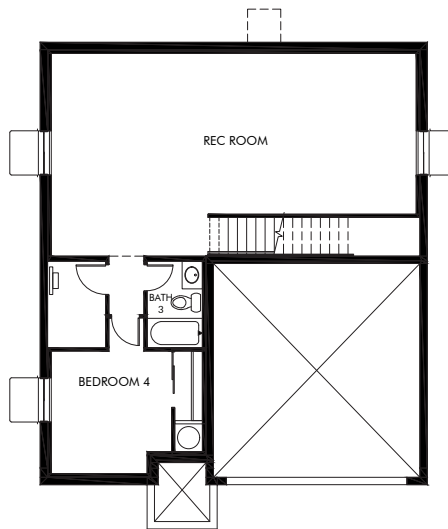
OPT. FINISHED BASEMENT
