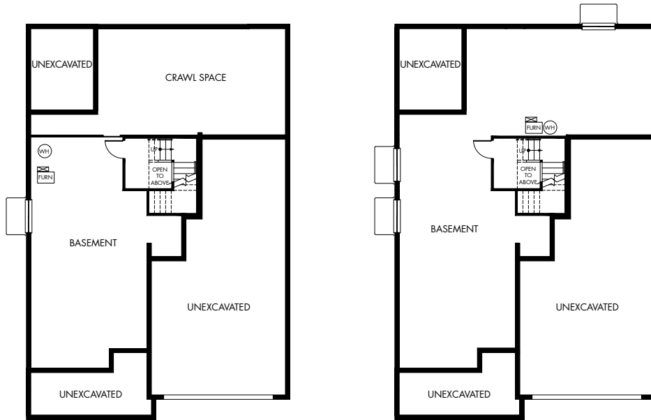
STANDARD BASEMENT
