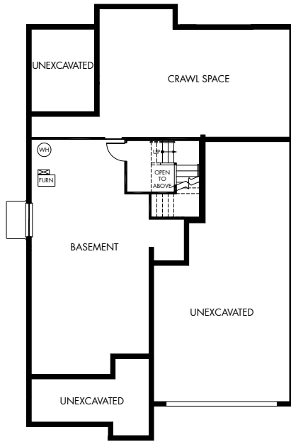
STANDARD BASEMENT
