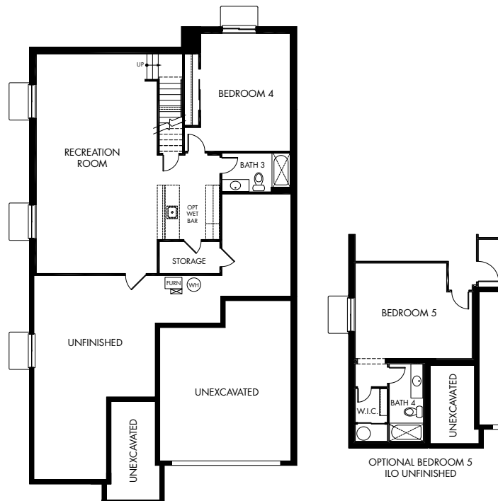
STANDARD BASEMENT
