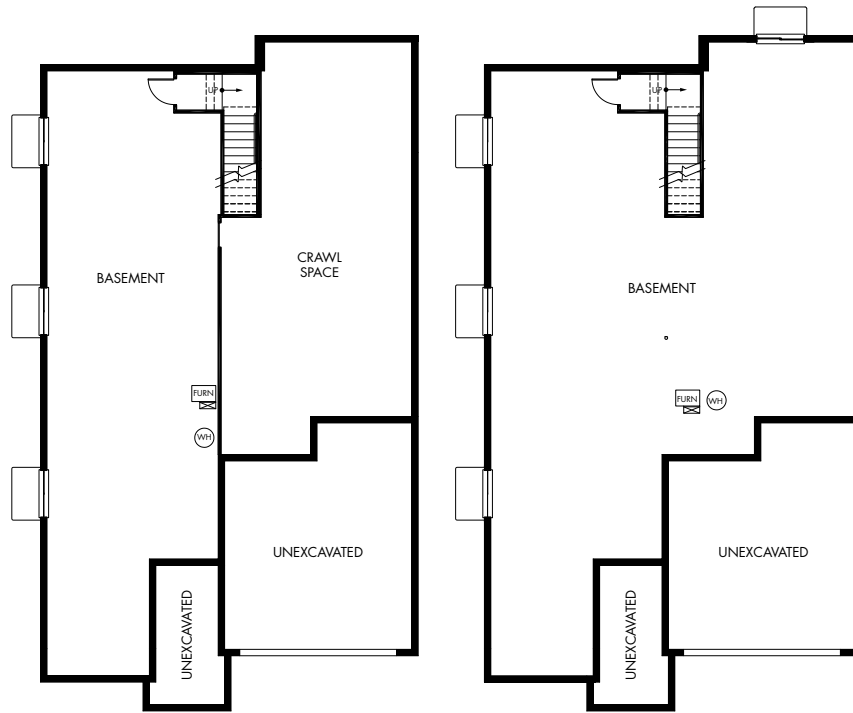
STANDARD BASEMENT
