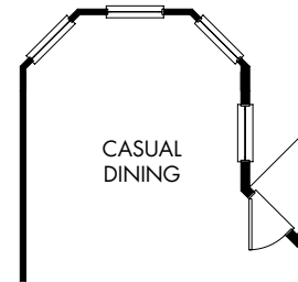
⑥ OPT. BAY WINDOW AT CASUAL DINING (BAY0008)
