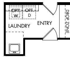
⑤ OPT. FREESTANDING LAUNDRY SINK (PLM0178)
