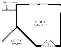
OPT. STUDY ILO FLEX
