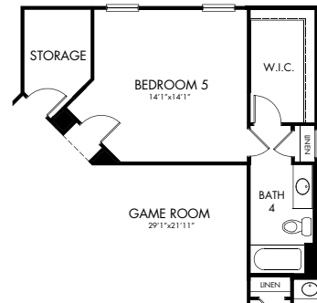
OPT. BEDROOM 5 AND BATH 4 ILO MEDIA ROOM
