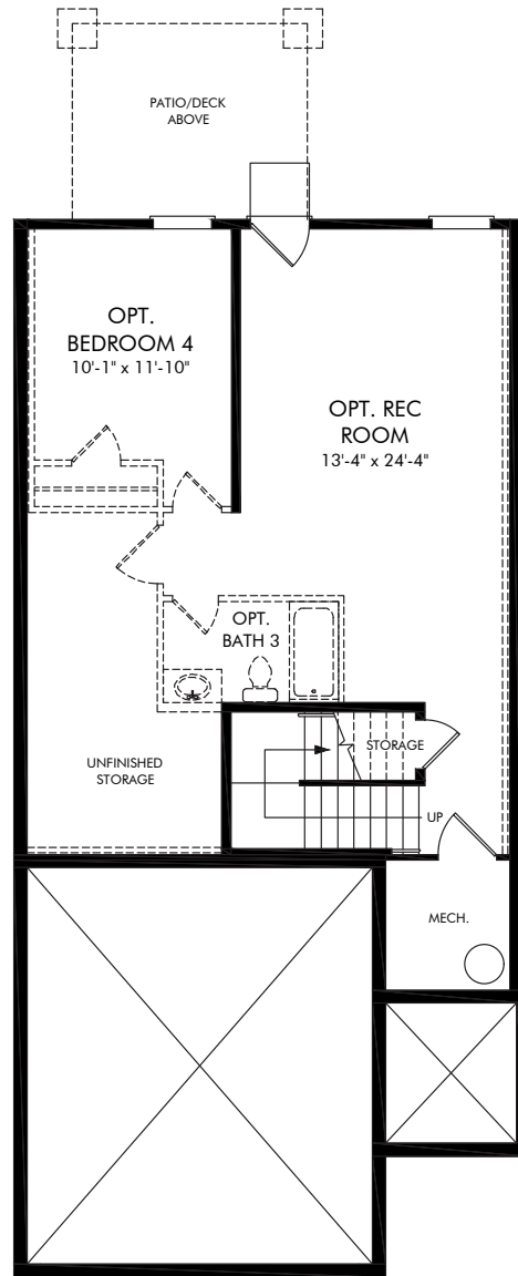
OPT. UNFINISHED BASEMENT W/OPT. FINISHED BEDROOM 4, BATH 3 & REC ROOM
