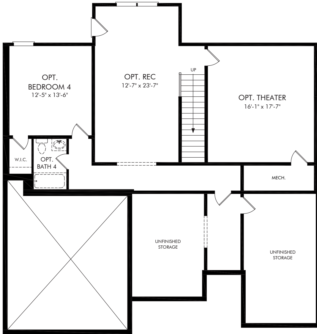
OPT. BASEMENT WITH OPT. REC, THEATER, BEDROOM 4 & BATH 4
