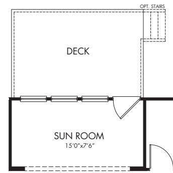
OPT. DECK AT SUN ROOM
