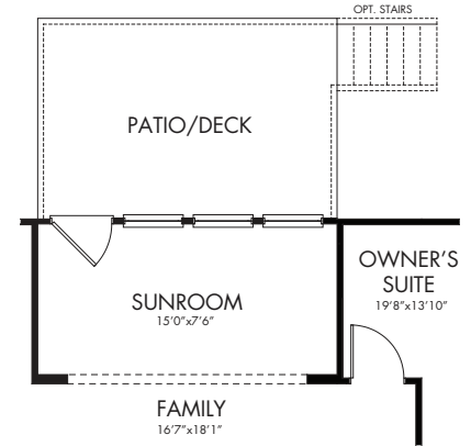
OPT. SUNROOM
