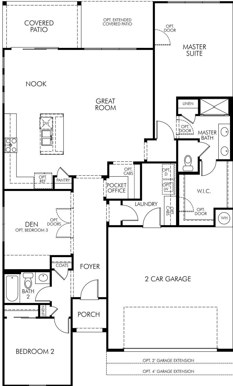
FLOOR PLAN
